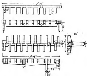
Figs. 567-571. Finger Grate Bars.
